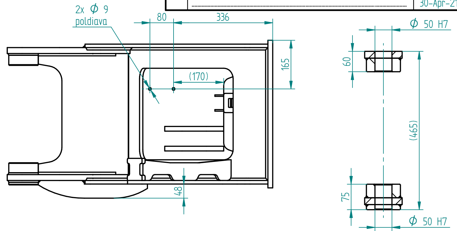
SECTION F-F
