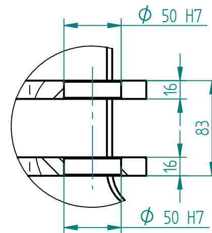
DETAIL G
