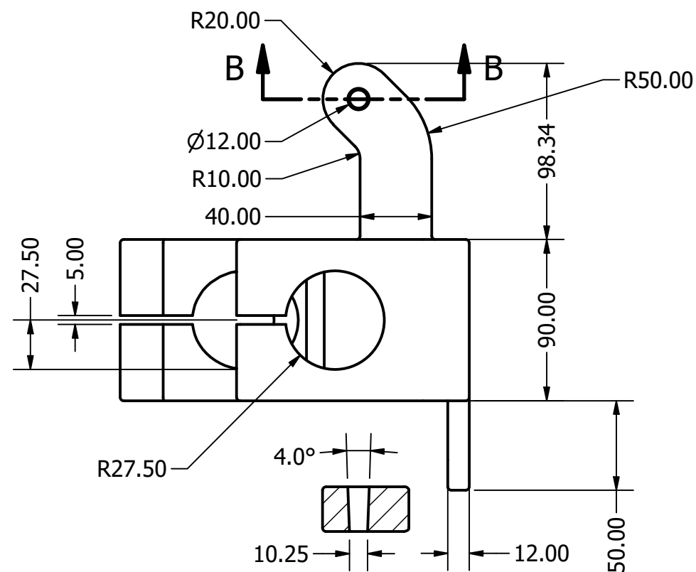
SECTION B-B SCALE 1 / 3
